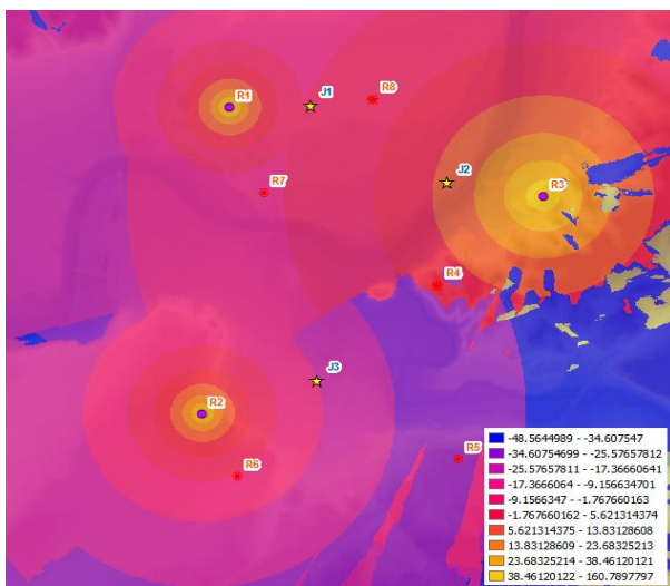
Monostatic radar coverage
