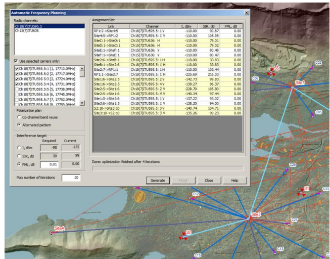
Automated Frequency planning for microwave network
